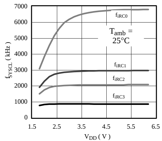
Figure 55. f_{SYSCL} = f(V_{DD}) ; internal RC
