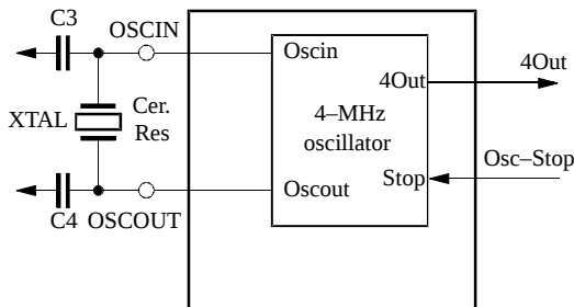
Figure 15. System clock oscillator
